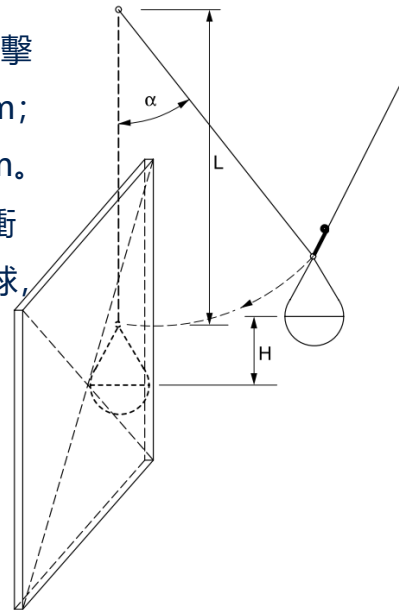
Figure 2 – Impact on vertical assembly h = drop height; L = length rope; \alpha = 65°
